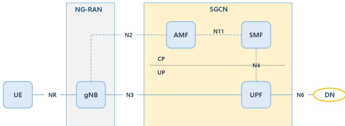
Figure 4: 5GC CUPS structure
