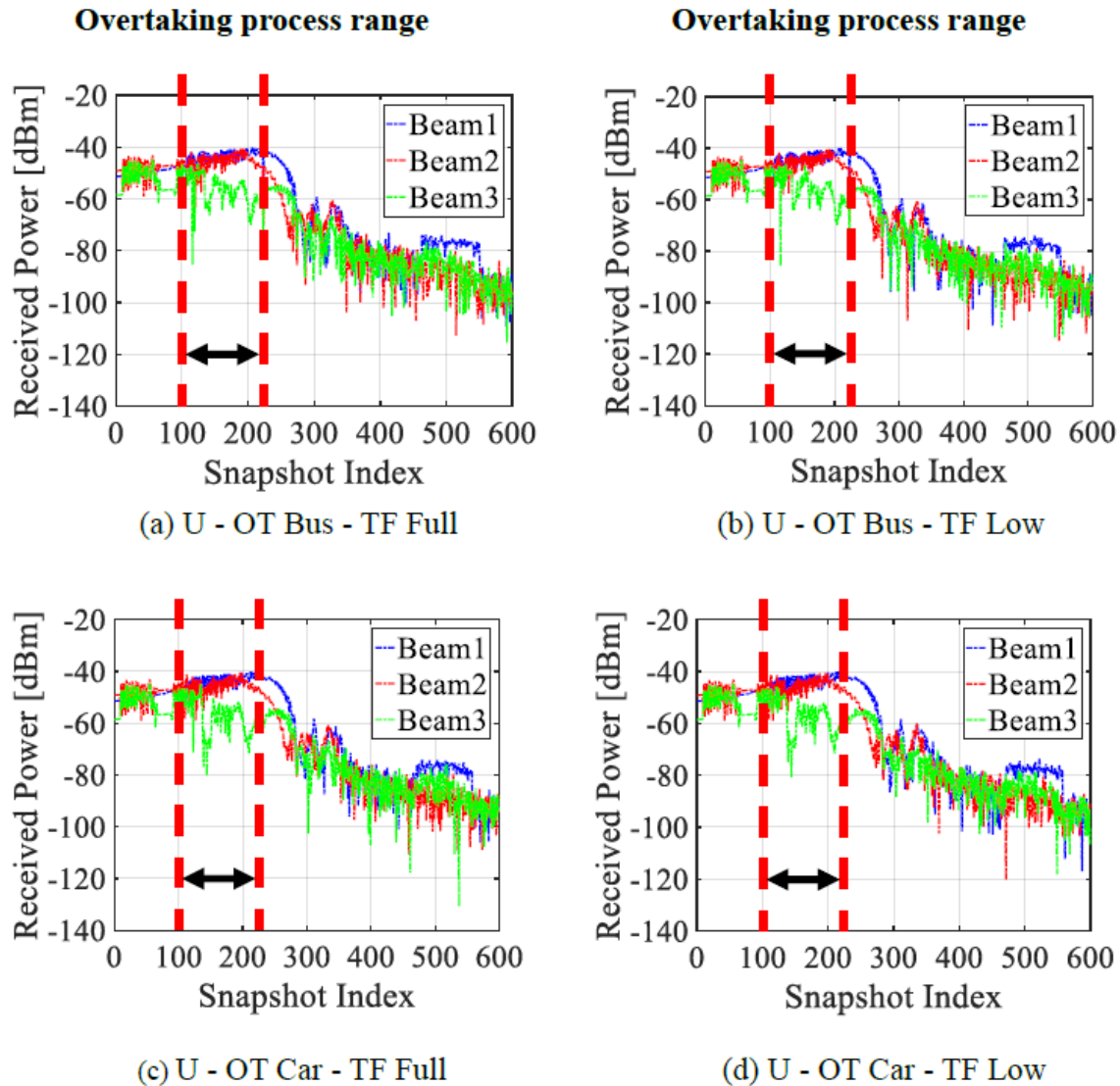
Figure 15: Received power of the overtaking situation in the urban scenario
