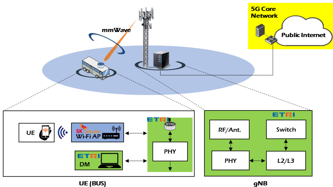
Figure 3: Architecture of Korean 5G cellular access testbed
