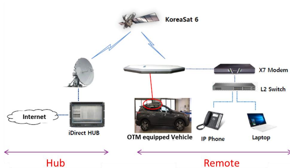
Figure 26: The components of the KSAT consisting of the hub and remote sides
