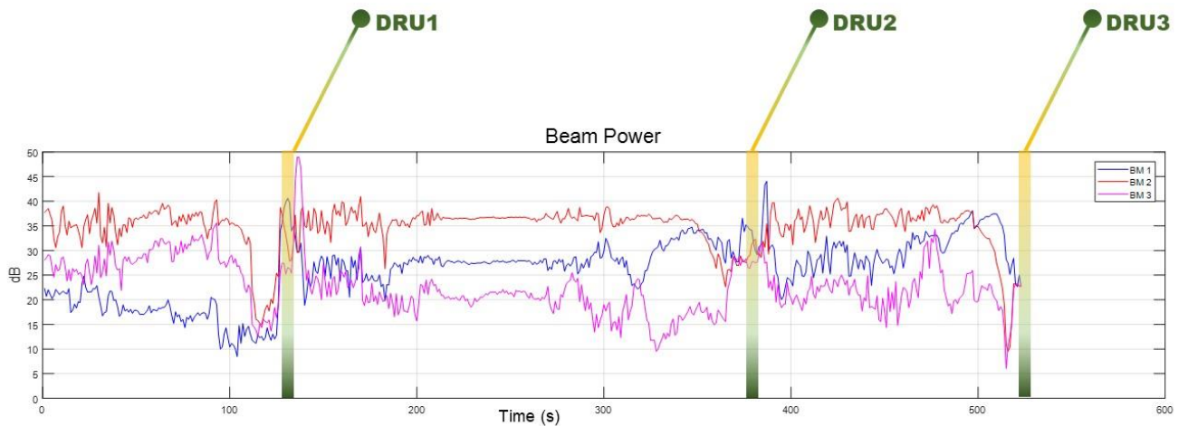
Figure 17: Received power for TE beam 1, 2, 3
