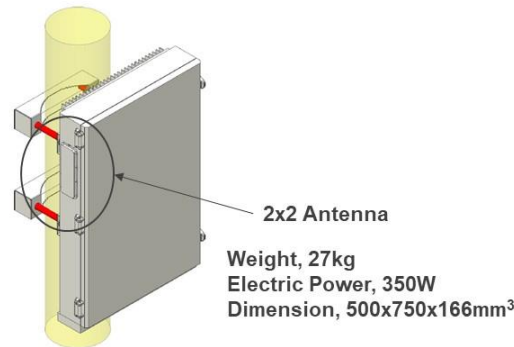
Figure 9: Image of the DRU case
