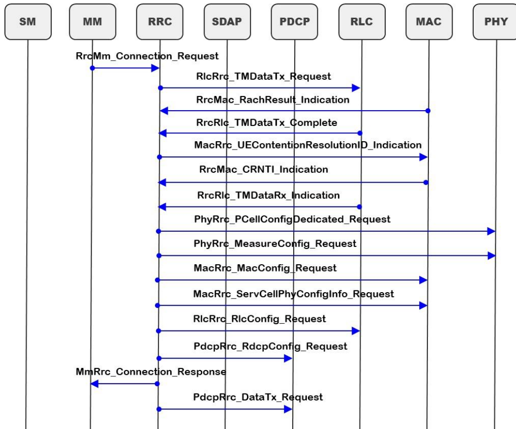
Figure 22: flow chart for an RRC connection setup
