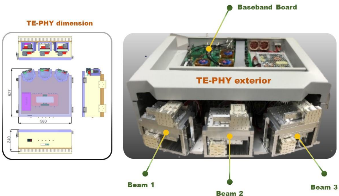
Figure 12: TE-PHY exterior and dimension
