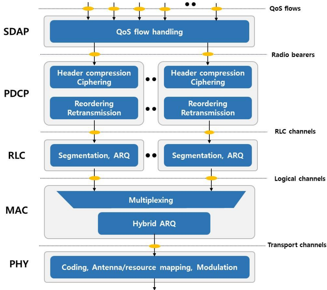
Figure 7: User-plane protocol stacks for downlink
