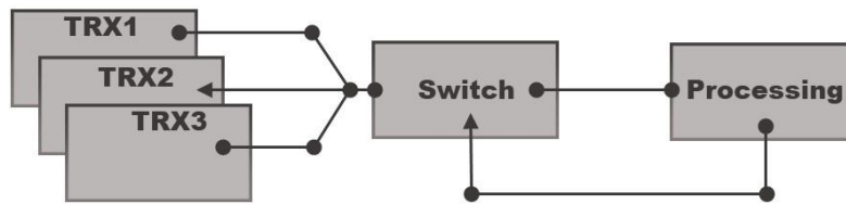
Figure 13: Beam switching process
