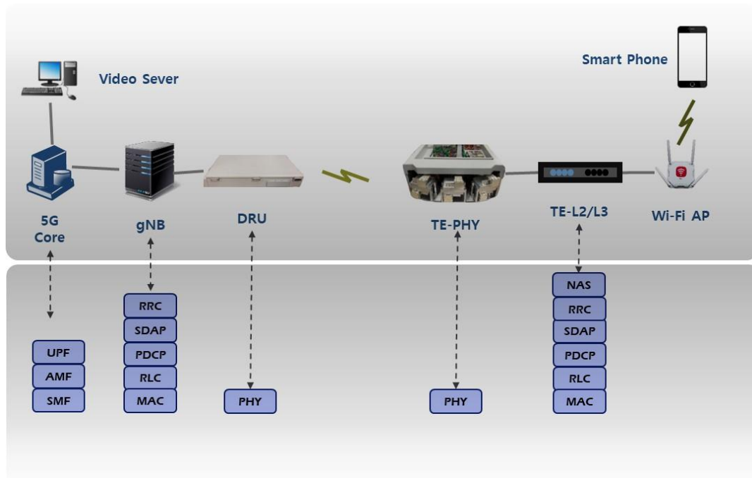
Figure 8: Component HW and protocol stacks of the 5G CATB
