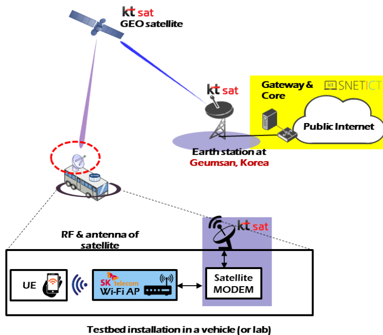
Figure 25: Conceptual diagram of the Korean satellite access testbed
