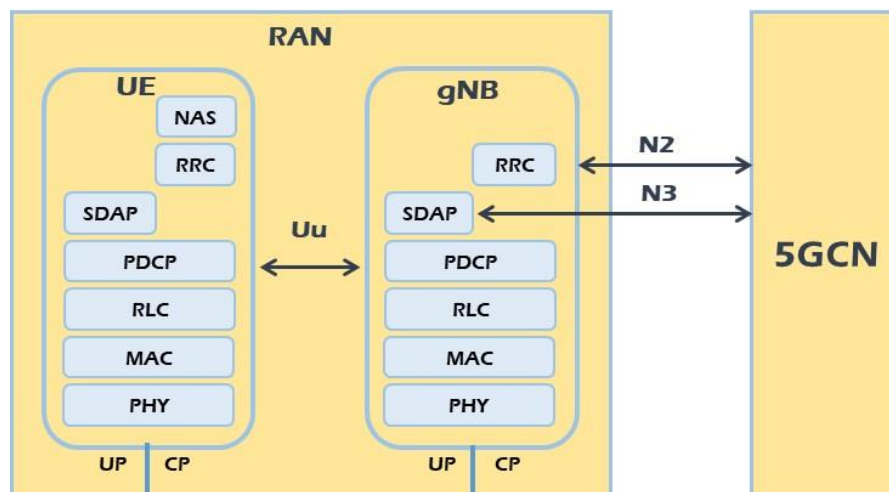
Figure 6: Architecture of the RAN
