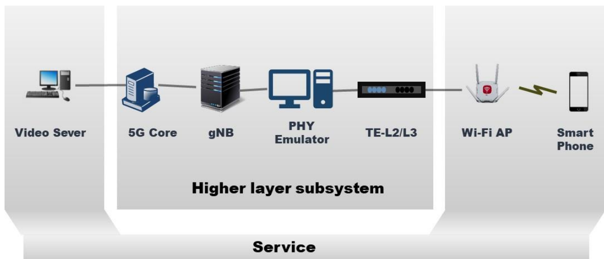
Figure 21: Higher layer subsystem test setup
