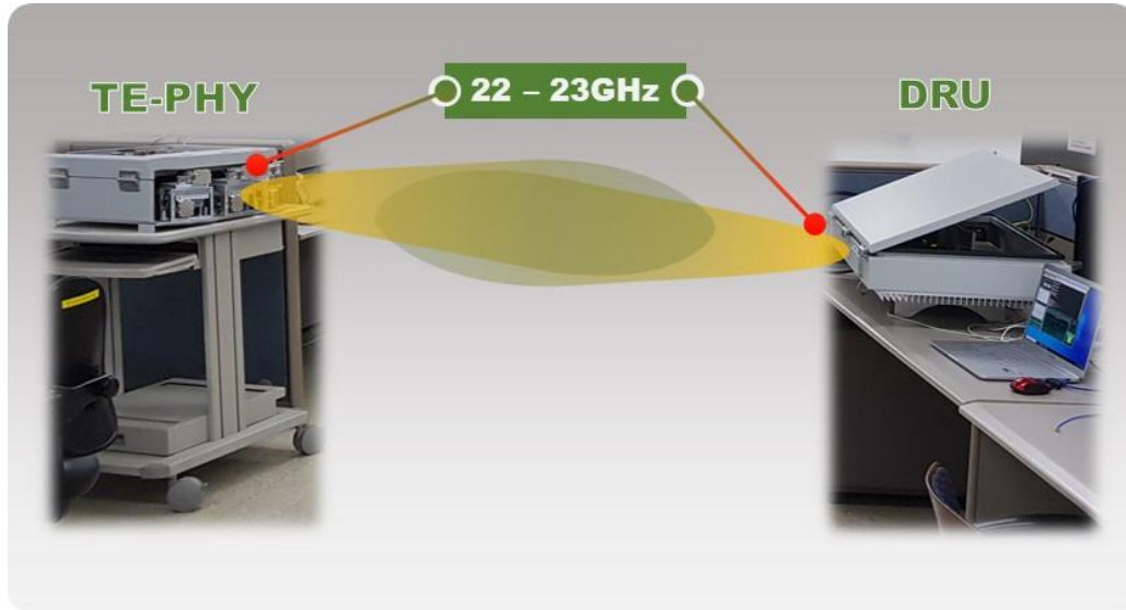
Figure 18: Physical layer subsystem test setup
