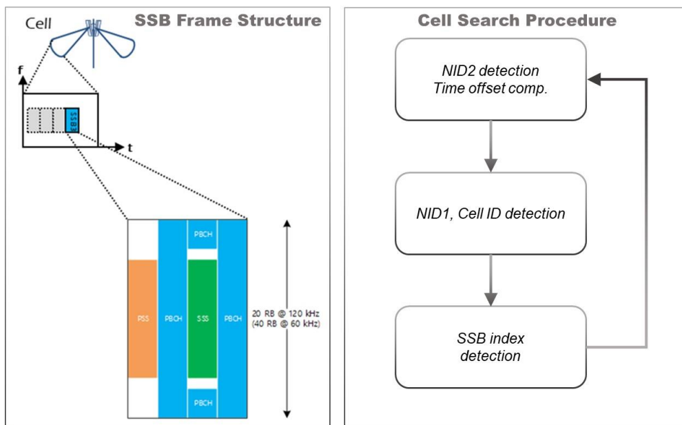
Figure 19: SSB frame structure and cell search procedure
