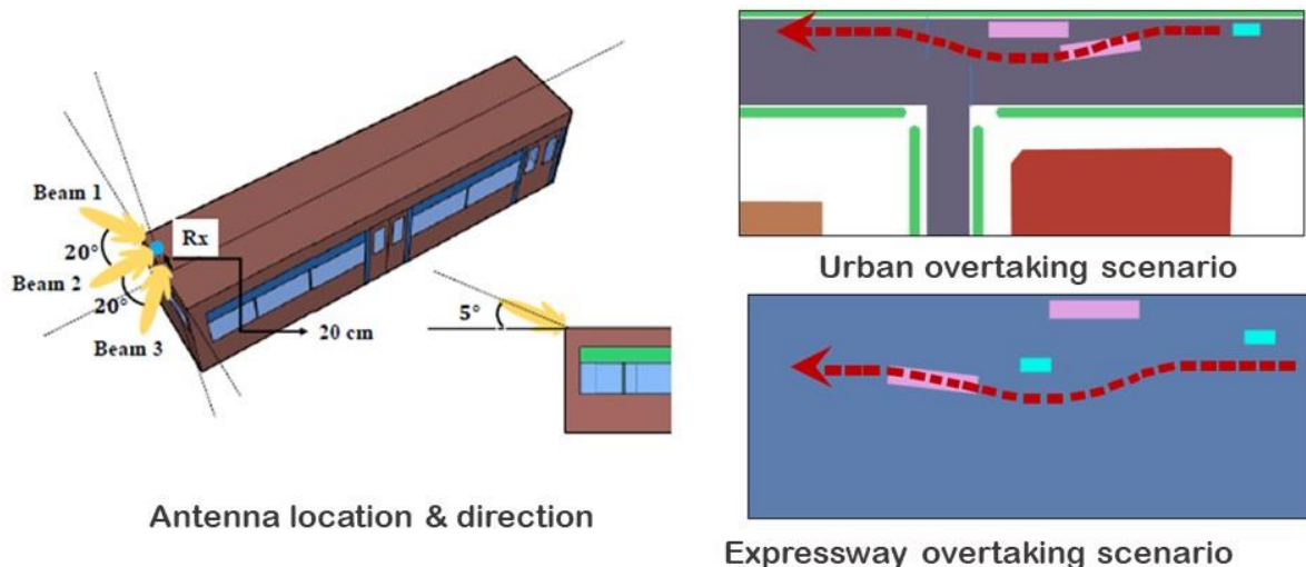
Figure 14: Beam switching simulation scenario
