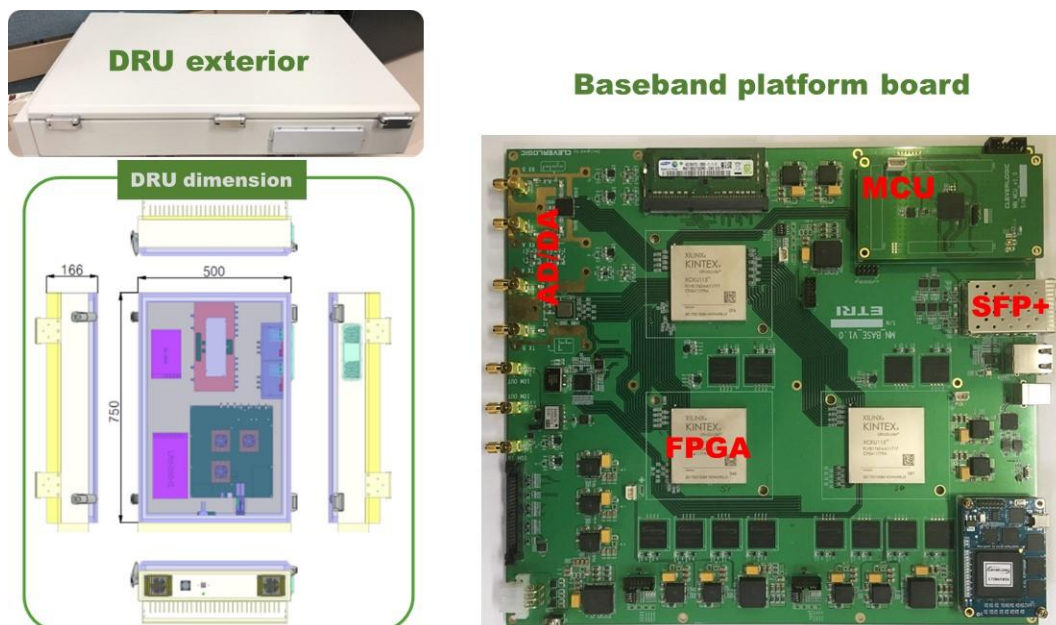
Figure 10: Pictures of a DRU case and DU board
