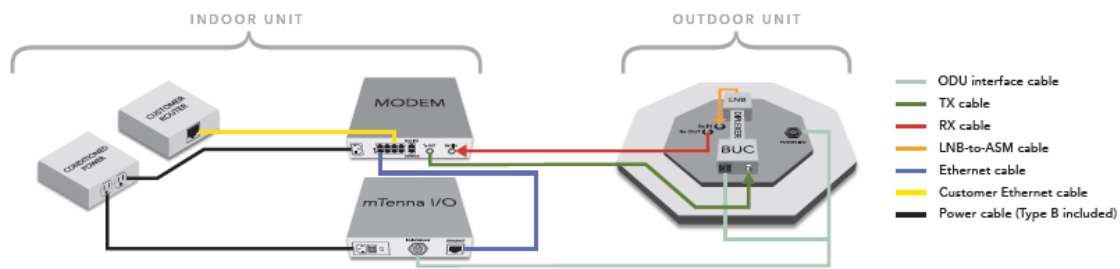
Figure 27: Components of the Kymeta ASM
