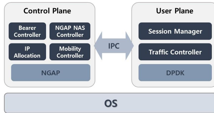
Figure 5: Functional diagram of the 5GCN
