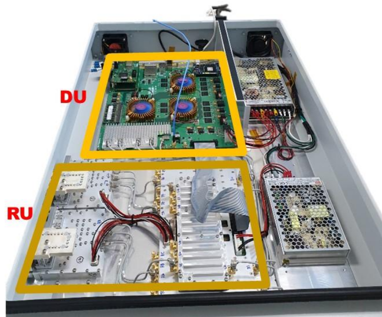
Figure 11: Picture of DRU interior
